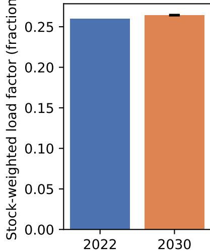
Load factor
